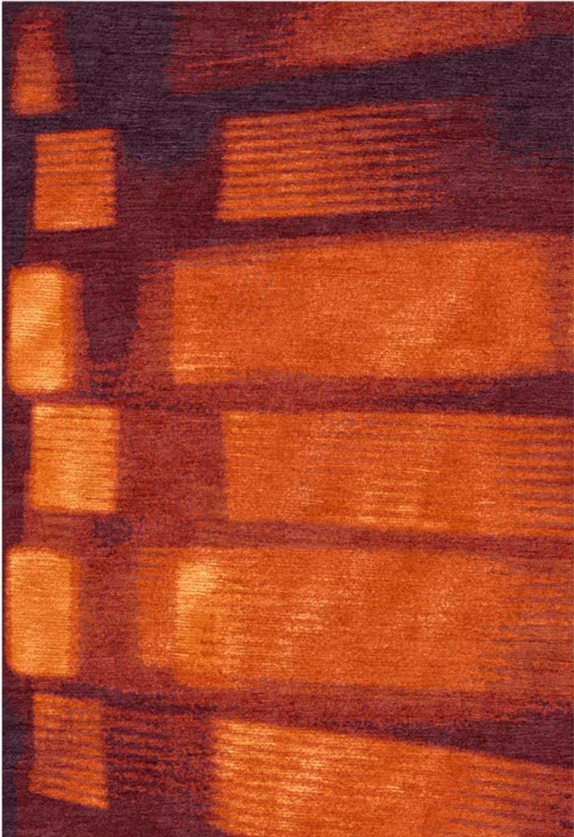
Haze in TJ 2002 Burgundy
